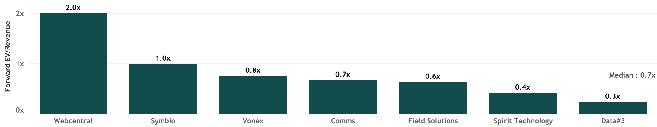
EV/Jun-24 Rev
