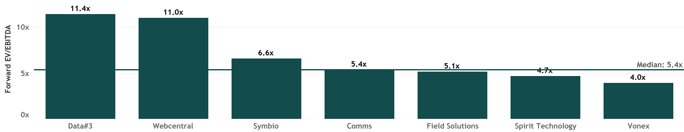
EV/Jun-24 EBITDA
